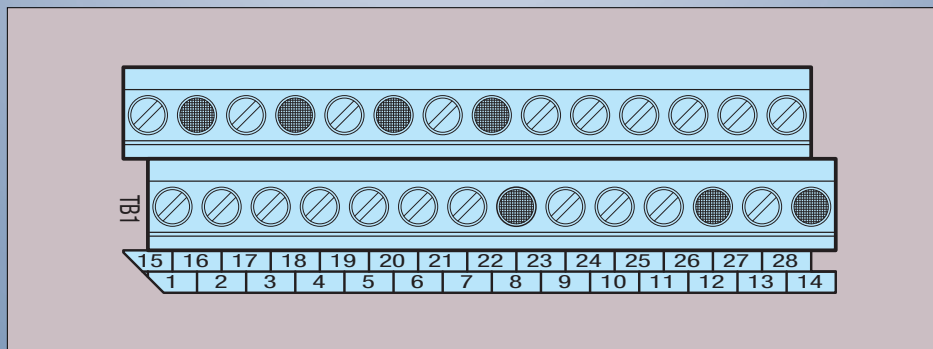
FIGURE 2 – IODA TERMINAL BLOCK TB1 LAYOUT
